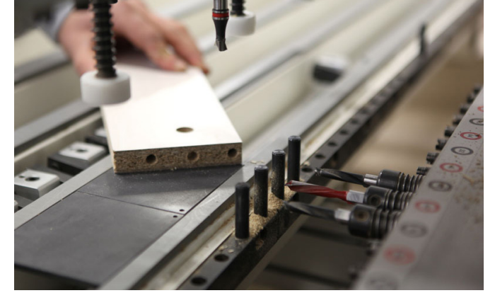
MİNİFİX DELİK İŞLEMLERİ (MINIFIX HOLE OPERATIONS)
